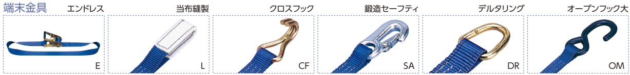
写真:品番LBR100 CF5-40CF
